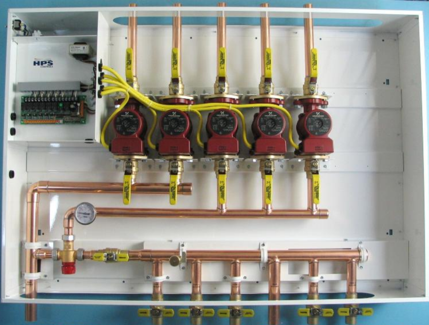
CFV-523 [Combo Temp Mixing Valve 2-Hi, 3-Lo Zone Control Station]
